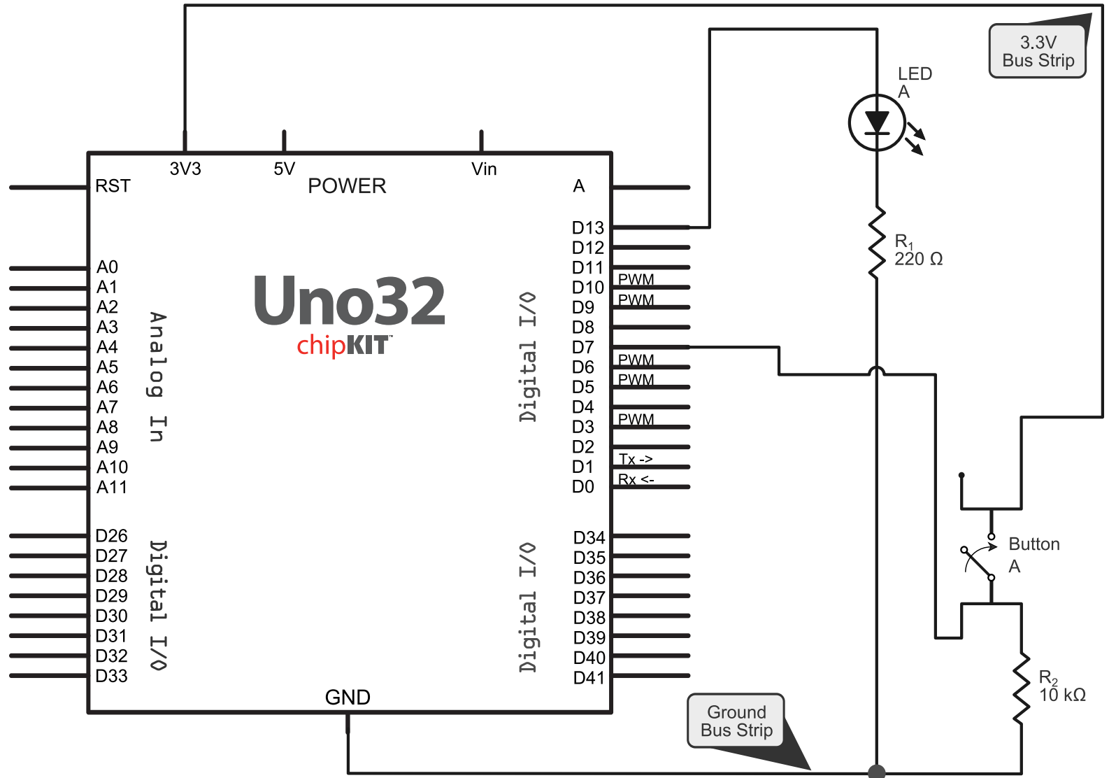
Button-Controlled LED
