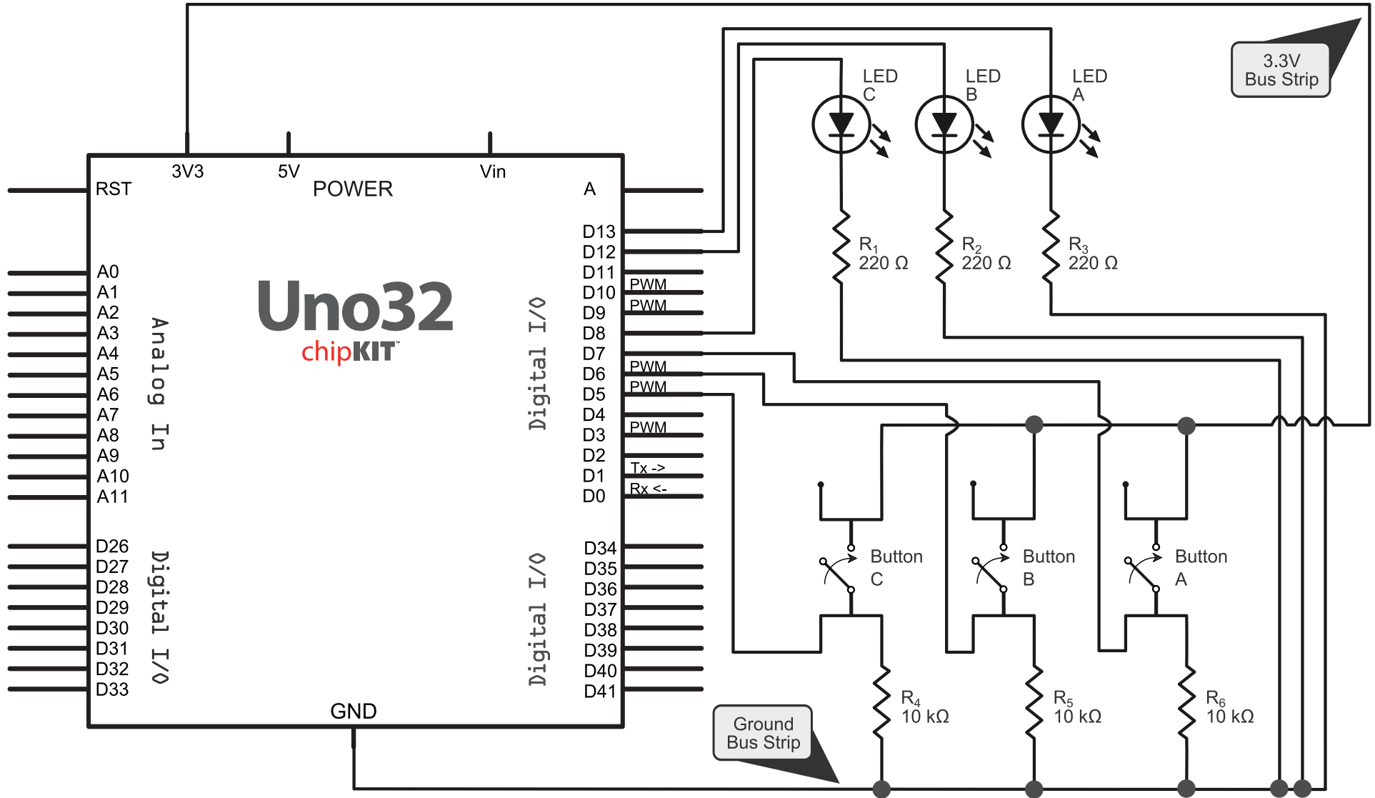
Button-Controlled LEDs
