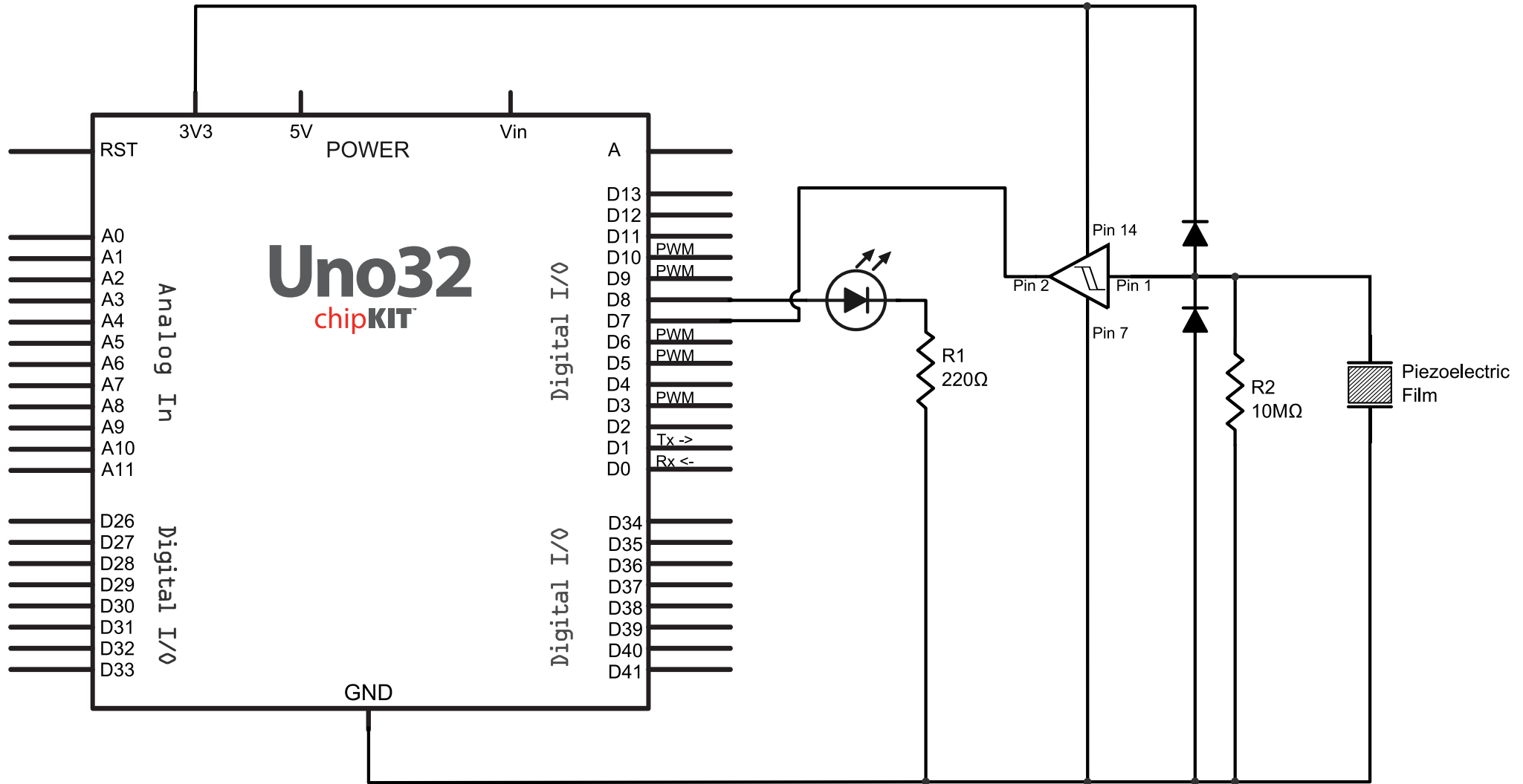
Piezoelectric Switch
